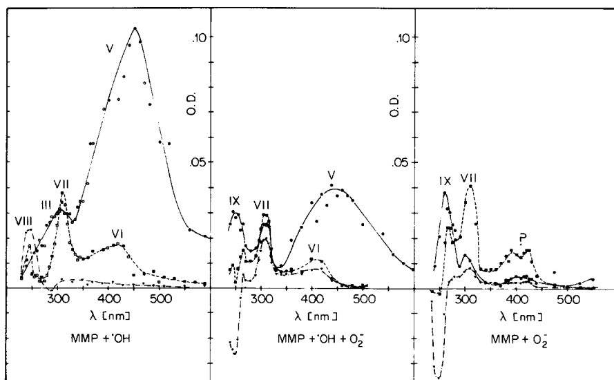
Figure 1 a-c: Transient spectra of MMP ( 6.3 \times 10^{-3} M) at pH 6.8 (a) solutions saturated with N_2O ; (b) solutions saturated with O_2 ; (c) solutions saturated with O_2 , formate ( 5 \times 10^{-2} M) added; solid lines (●): 10 \mu sec after the pulse; dashed lines (■): 100 \mu sec after the pulse; dotted lines (▼): 1 msec (b), resp. 10 msec (a,c) after the pulse.
